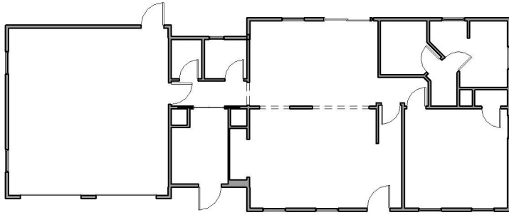
① Lvl1 Org. 3/32" = 1'-0"
