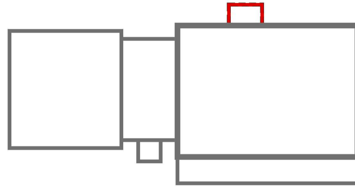
② BM Demo 3/32" = 1'-0"
